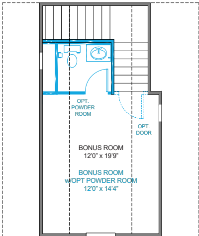
STANDARD BONUS ROOM w/OPT POWDER ROOM PLAN 1411 ADDS 4' TO FRONT OF GARAGE
