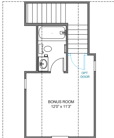
BONUS ROOM w/FULL BATH PLAN 1411 ADDS 4' TO FRONT OF GARAGE
