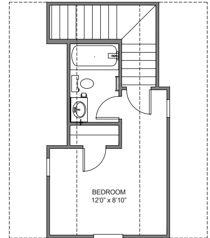
BEDROOM PLAN 1411 ADDS 4' TO FRONT OF GARAGE
