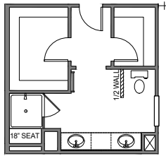
LUXURY SHOWER OPT. 1 42"x42" FRAMED TILE SHOWER BASE TILE WALLS w/18" TILE SEAT
