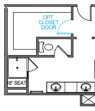
ALT. MASTER BATH 2 LUXURY SHOWER OPT 1 42"x42" FRAMED TILE SHOWER BASE TILE WALLS w/18" TILE SEAT
