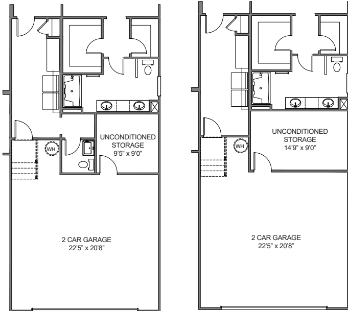
UNCONDITIONED STORAGE w/POWDER ROOM PULLS GARAGE FORWARD 10'0"
