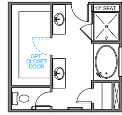
LUXURY BATH OPT 3 42"x60" GARDEN TUB w/CERAMIC TUB SURROUND 42"x48" FRAMED TILE SHOWER BASE TILE WALLS w/12" TILE SEAT
