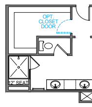
ALT. MASTER BATH 2 LUXURY SHOWER OPT 2 42"x48" FRAMED TILE SHOWER BASE TILE WALLS w/12" TILE SEAT
