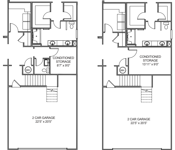
CONDITIONED STORAGE w/POWDER ROOM PULLS GARAGE FORWARD 9'0"
