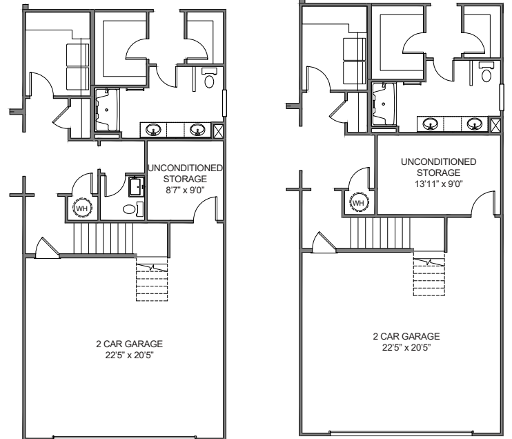
UNCONDITIONED STORAGE w/POWDER ROOM PULLS GARAGE FORWARD 9'0"
