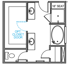
LUXURY BATH OPT 2 42"x60" GARDEN TUB w/CERAMIC TUB SURROUND 42"x42" PRE-FORM SHOWER PAN TILE WALLS w/18" TILE SEAT
