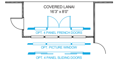
GREAT ROOM BACK WALL OPTIONS
