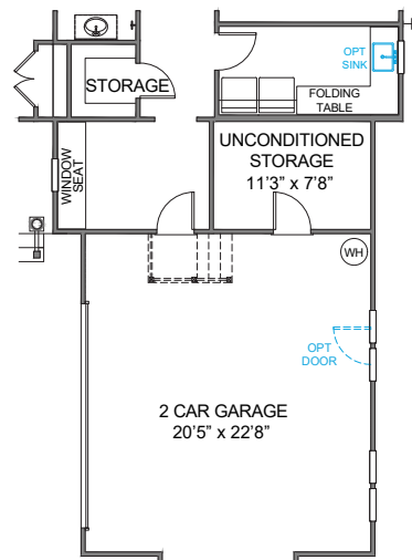
UNCONDITIONED STORAGE PLAN 2782
