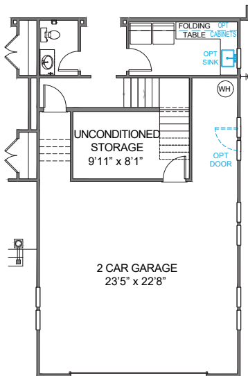
UNCONDITIONED STORAGE PLAN 2781 PULLS GARAGE FORWARD 1'0"
