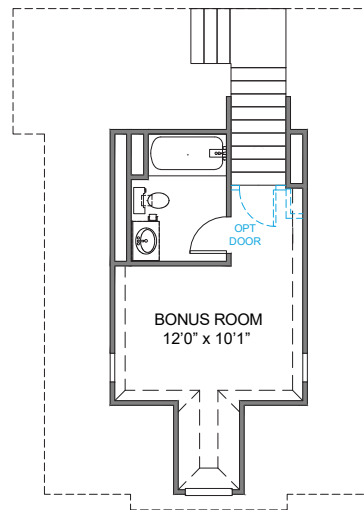
BONUS ROOM w/FULL BATH PLAN 2783 ELEVATIONS D-C1
