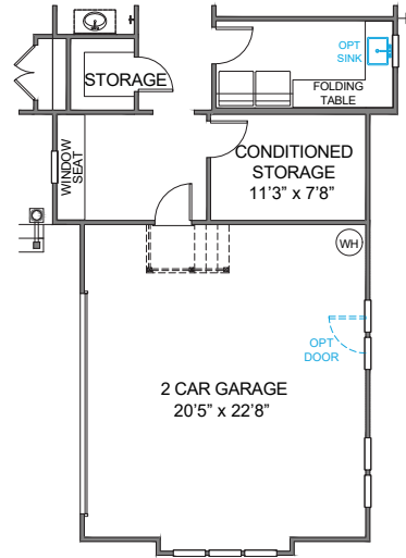
CONDITIONED STORAGE PLAN 2782
