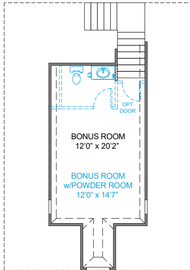
BONUS ROOM PLAN 2781 ELEVATIONS D-C1
