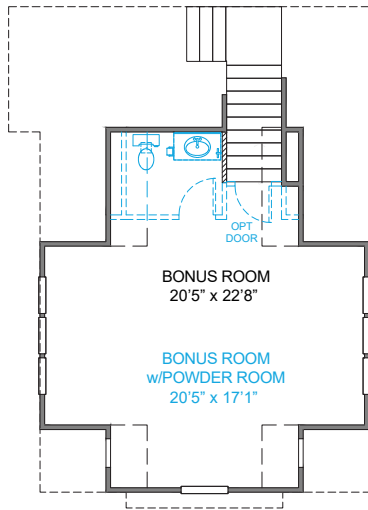
BONUS ROOM PLAN 2783 ELEVATIONS D-A1 & D-B1
