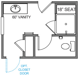
LUXURY SHOWER OPT 1 42" x 42" PRE-FORM SHOWER PAN TILE WALLS w/18" TILE SEAT
