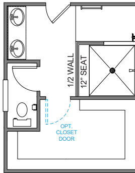
CUSTOM SHOWER OPTION 3
