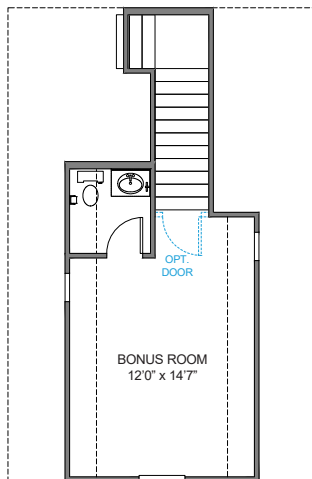
BONUS ROOM w/POWDER ROOM PLAN 1403
