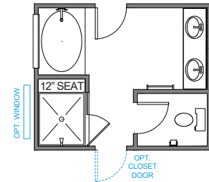
LUXURY BATH OPT 3 42" x 60" GARDEN TUB w/CERAMIC TUB SURROUND 42" x 48" FRAMED TILE SHOWER BASE TILE WALLS w/12" TILE SEAT REDUCES WIC BY 1'9"
