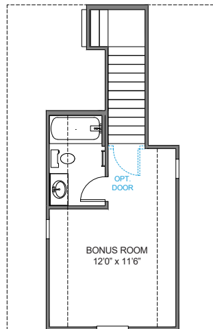
BONUS ROOM w/FULL BATH PLAN 1403
