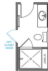
LUXURY SHOWER OPT 2 42" X 48" FRAMED TILE SHOWER BASE TILE WALLS w/12" TILE SEAT
