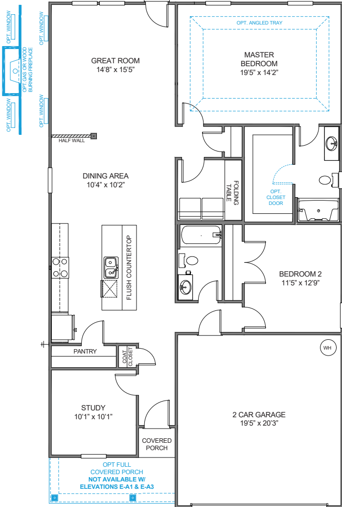
Plan 1548
