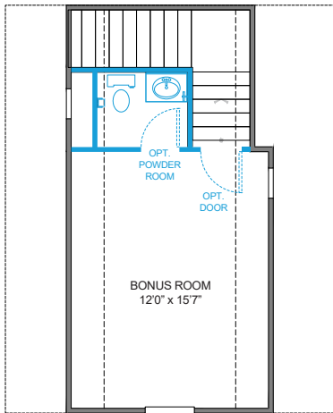
STANDARD BONUS ROOM w/OPT POWDER ROOM PLAN 1549
