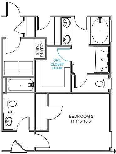
LUXURY BATH OPT 1 42" X 60" GARDEN TUB 35" X 60" FIBERGLASS SHOWER UNIT LOSE 4" FROM WIDTH AND 2'4" FROM DEPTH OF BEDROOM 2
