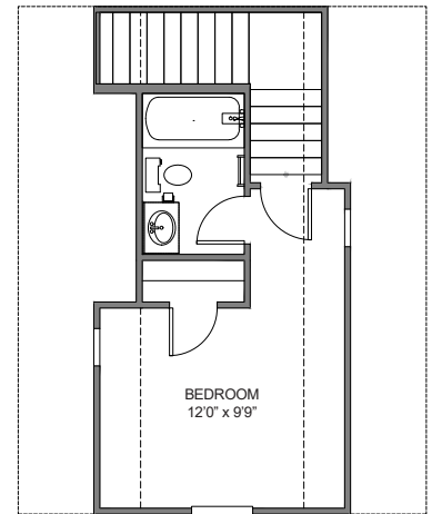
BEDROOM PLAN 1549
