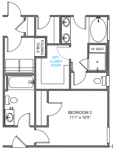
LUXURY BATH OPT 2 42" X 60" GARDEN TUB w/CERAMIC TUB SURROUND 42" X 42" PRE-FORM SHOWER PAN TILE WALLS w/18" TILE SEAT LOSE 4" FROM WIDTH AND 2'4" FROM DEPTH OF BEDROOM 2
