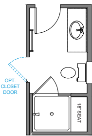
LUXURY SHOWER OPT 1 42" X 42" PRE-FORM SHOWER PAN TILE WALLS w/18" TILE SEAT
