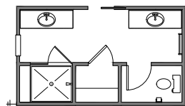
ALT MASTER BATH 2 w/LUXURY SHOWER OPT 2 42" x 48" FRAMED TILE SHOWER BASE TILE WALLS w/12" TILE SEAT LOSE 4" FROM WIC 1 LOSE 2'10" FROM WIC 2
