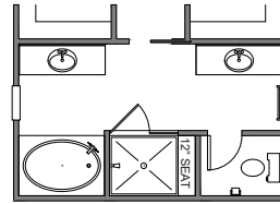
LUXURY BATH OPT 3 42" x 60" GARDEN TUB w/CERAMIC TUB SURROUND 42" x 48" FRAMED TILE SHOWER TILE WALLS w/12" TILE SEAT LOSE 4" FROM WIC 1 LOSE 2'10" FROM WIC 2
