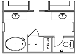
LUXURY BATH OPT 2 42" x 60" GARDEN TUB w/CERAMIC TUB SURROUND 42" x 42" PRE-FORM PAN TILE WALLS w/18" TILE SEAT LOSE 4" FROM WIC 1 LOSE 2'10" FROM WIC 2
