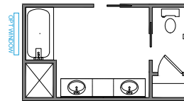
ALT MASTER BATH 1 w/TUB/SHOWER LOSE 2'6" FROM WIC
