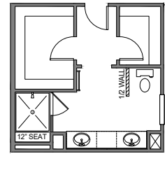
LUXURY SHOWER OPT. 2 42"x48" FRAMED TILE SHOWER BASE TILE WALLS w/12" TILE SEAT
