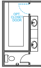
LUXURY BATH - ENLARGED VANITY OPT 42"x60" GARDEN TUB 35"x60" FIBERGLASS SHOWER UNIT
