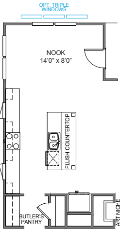
ALTERNATE KITCHEN 1 NA w/BEDROOM 3 PRIVATE BATH OPTION
