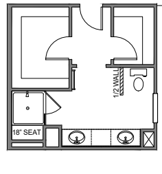
LUXURY SHOWER OPT. 1 42"x42" FRAMED TILE SHOWER BASE TILE WALLS w/18" TILE SEAT
