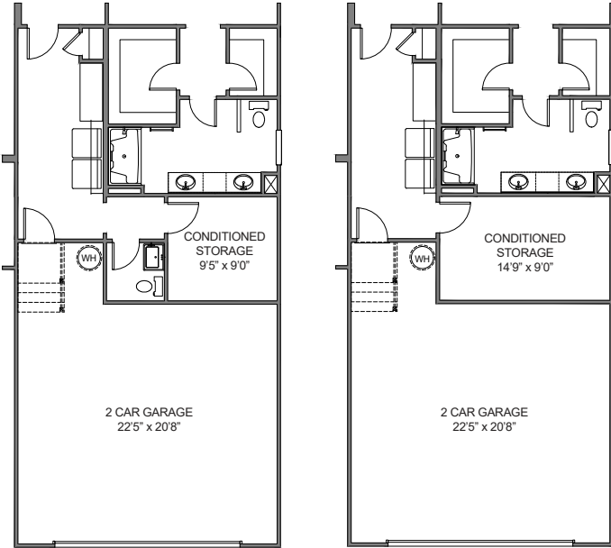
CONDITIONED STORAGE w/POWDER ROOM PULLS GARAGE FORWARD 10'0"
