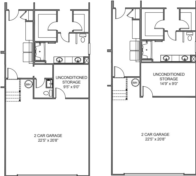
UNCONDITIONED STORAGE w/POWDER ROOM PULLS GARAGE FORWARD 10'0"
