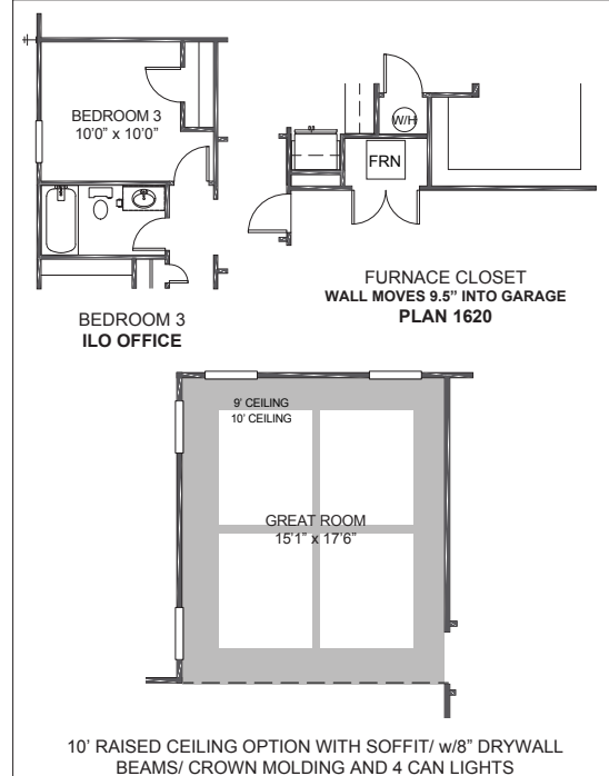
Main Floor Options
