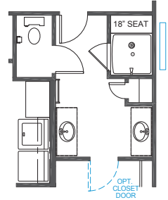
ALTERNATE MASTER BATH w/LUXURY SHOWER OPT 1 42"x42" PRE-FORMED SHOWER PAN 18" TILED SEAT & TILED WALLS
