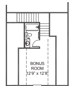
BONUS ROOM w/FULL BATH PLANS 1621 & 1623
