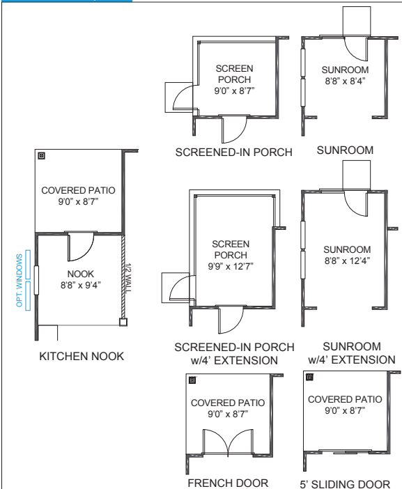
Kitchen Nook Options
