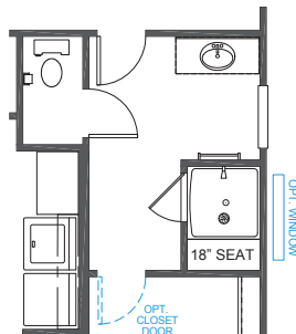
LUXURY SHOWER OPT 1 42"x42" PRE-FORMED SHOWER PAN 18" TILED SEAT TILED WALLS
