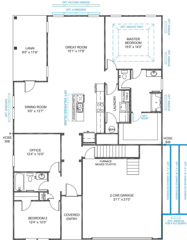
Main Floor Options
