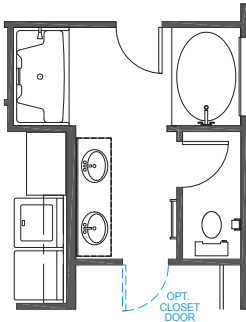
LUXURY MASTER BATH OPT 1 34" x 60" VIKRELL SHOWER 42" x 60" GARDEN TUB
