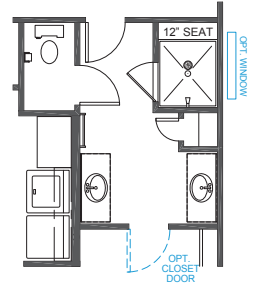
ALTERNATE MASTER BATH w/LUXURY SHOWER OPT 2 42"x48" FRAMED TILE SHOWER PAN 12" TILED SEAT & TILED WALLS
