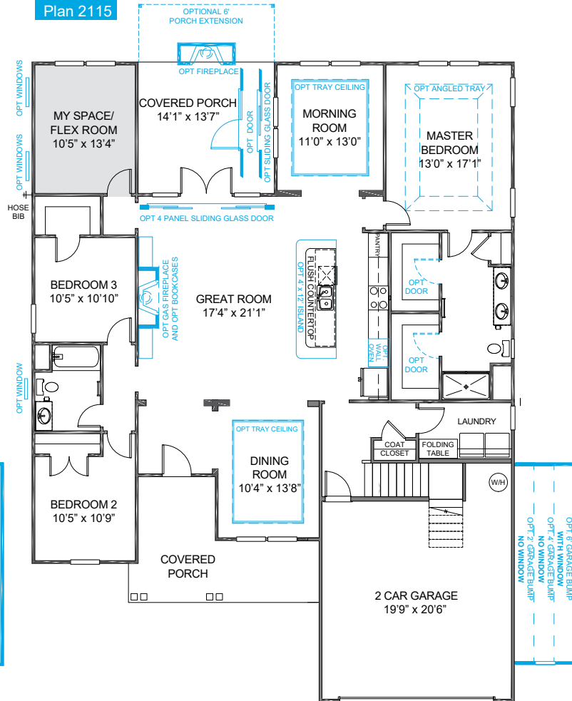
1st Floor Options
