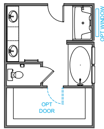
LUXURY BATH OPT 4 42" X 72" GARDEN TUB 34" X 60" VIKRELL SHOWER
