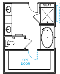
LUXURY BATH OPT 6 42" X 72" GARDEN TUB 42" X 48" TILE PAN 12" TILE SEAT & WALLS
