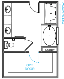
LUXURY BATH OPT 1 42" X 60" GARDEN TUB 34" X 60" VIKRELL SHOWER
