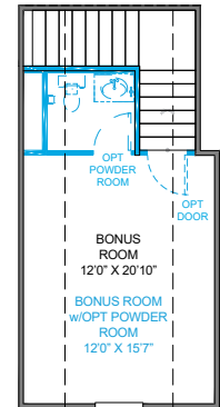
Plan 2113 - Std. Bonus Rm.
