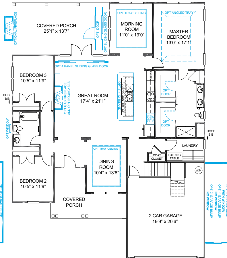
1st Floor Options
