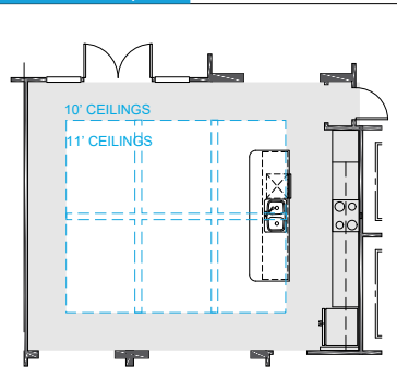
11' RAISED CEILING w/8" DRYWALL BEAMS & CROWN MOLDING
