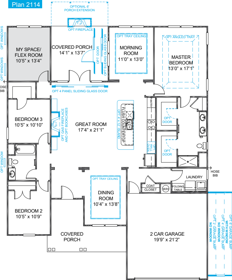
Plan 2114
