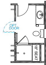
LUXURY SHOWER OPT 1 42" x 42" PRE-FORM SHOWER PAN TILE WALLS w/12" TILE SEAT
