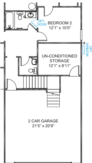
UN-CONDITIONED STORAGE w/POWDER ROOM PULLS GARAGE FORWARD 9'3" PLANS 1604 & 1606
