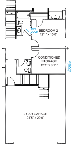
CONDITIONED STORAGE w/POWDER ROOM PULLS GARAGE FORWARD 9'3" PLANS 1605 & 1607
