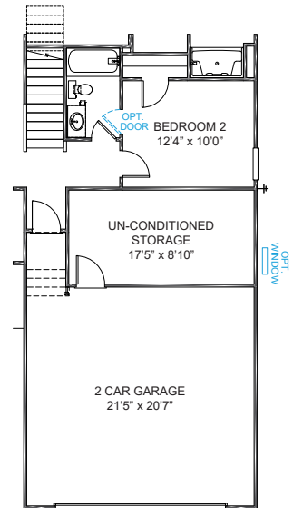
UN-CONDITIONED STORAGE PULLS GARAGE FORWARD 10' PLANS 1601 & 1603
