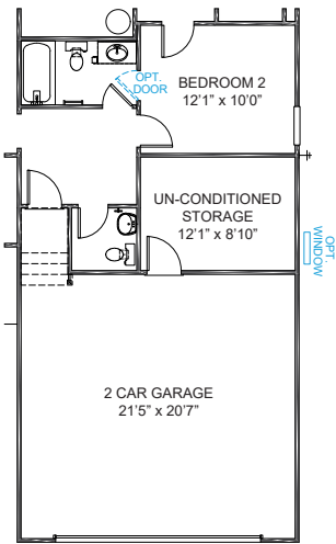
UN-CONDITIONED STORAGE w/POWDER ROOM PULLS GARAGE FORWARD 10' PLANS 1600 & 1602
