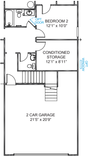
CONDITIONED STORAGE w/POWDER ROOM PULLS GARAGE FORWARD 9'3" PLANS 1604 & 1606
