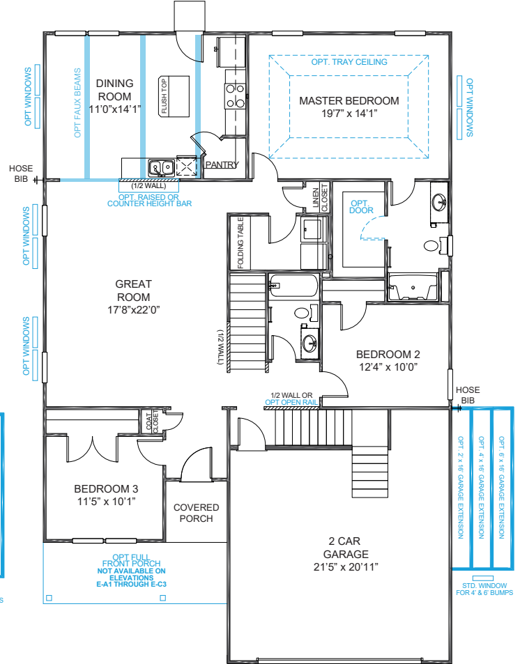
Plan 1605 (includes Garage Bonus Room)
