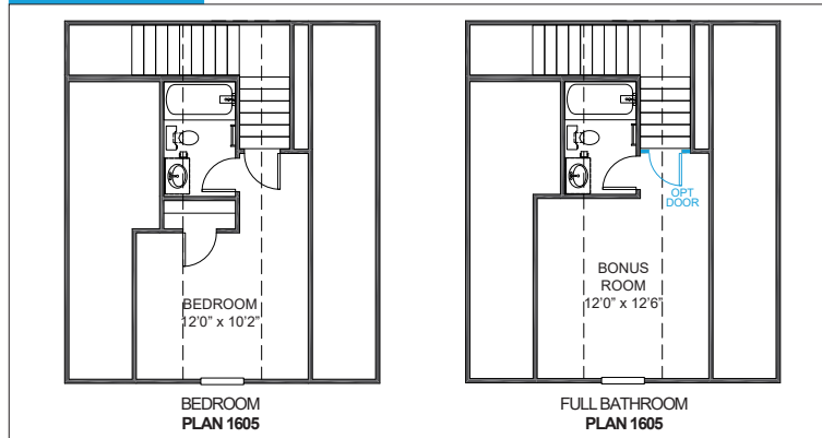
Hall Bath Options
