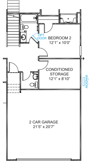
CONDITIONED STORAGE w/POWDER ROOM PULLS GARAGE FORWARD 10' PLANS 1601 & 1603
