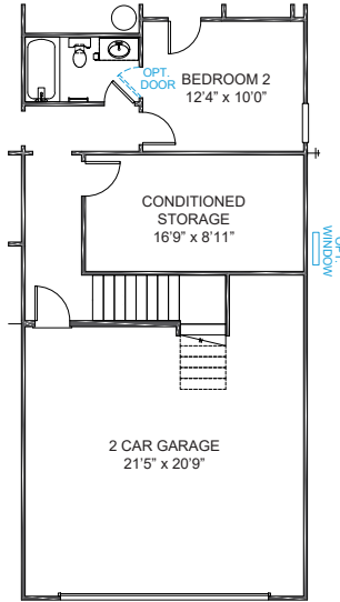
CONDITIONED STORAGE PULLS GARAGE FORWARD 9'3" PLANS 1604 & 1606
