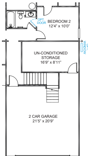
UN-CONDITIONED STORAGE PULLS GARAGE FORWARD 9'3" PLANS 1604 & 1606
