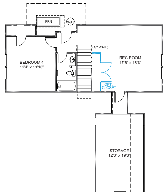
GUEST SUITE w/STORAGE AREA PLAN 1603
