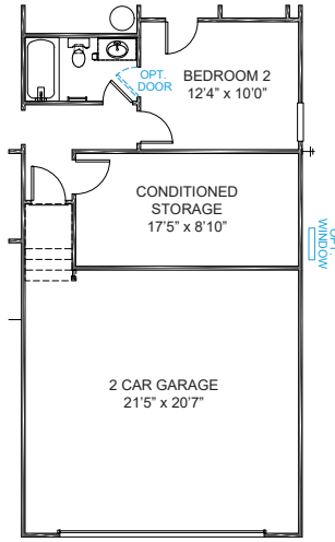
CONDITIONED STORAGE PULLS GARAGE FORWARD 10' PLANS 1600 & 1602
