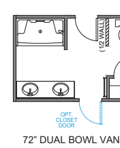
72" DUAL BOWL VANITY
