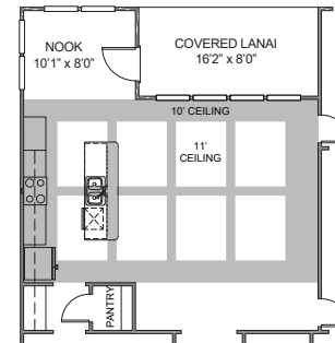
NOOK 10'1" x 8'0" COVERED LANAI 16'2" x 8'0" 11' RAISED CEILING w/SOFFIT/ 8" DRYWALL BEAMS/ CROWN MOLDING & 8 CAN LIGHTS (NOT AVAILABLE w/HP ROOF OR PLAN 1755 / 1757)
