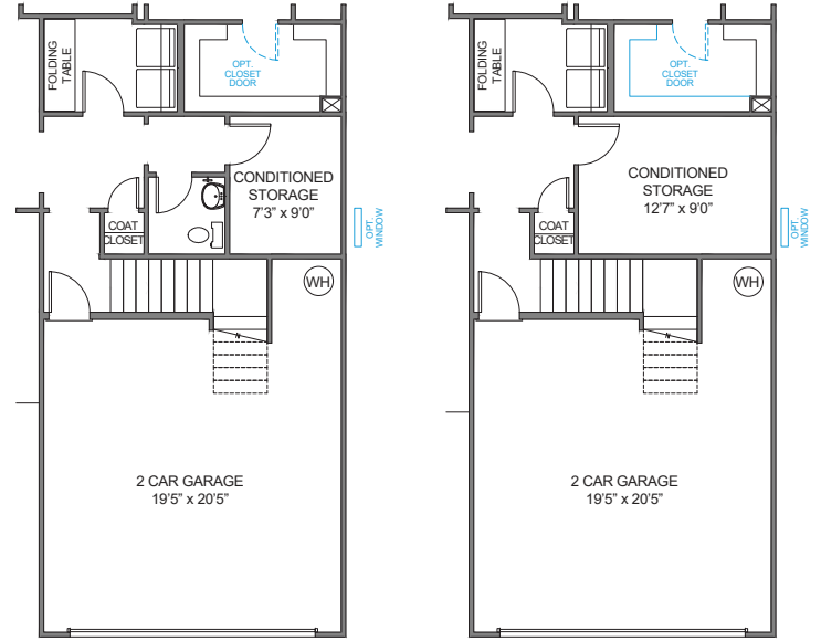
CONDITIONED STORAGE w/POWDER ROOM PULLS GARAGE FORWARD 9'0"
