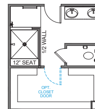
CUSTOM SHOWER OPTION 3
