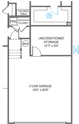
UNCONDITIONED STORAGE PULLS GARAGE FORWARD 10'0"
