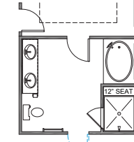
LUXURY BATH OPT 3 42" x 60" GARDEN TUB w/CERAMIC TUB SURROUND 42" x 48" FRAMED TILE SHOWER TILE WALLS w/12" TILE SEAT LOSE 2' FROM MASTER BR
