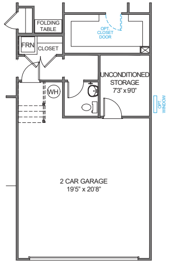
UNCONDITIONED STORAGE w/POWDER ROOM PULLS GARAGE FORWARD 10'0"
