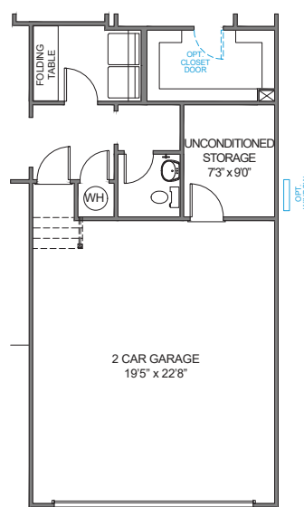
UNCONDITIONED STORAGE w/POWDER ROOM PULLS GARAGE FORWARD 12'0"
