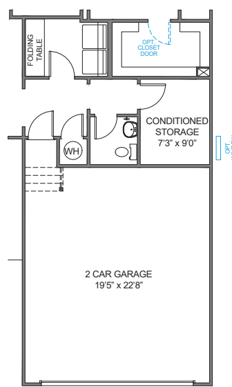
CONDITIONED STORAGE w/POWDER ROOM PULLS GARAGE FORWARD 12'0"
