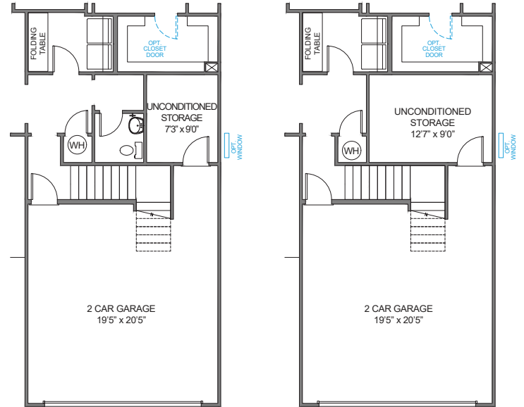
UNCONDITIONED STORAGE w/POWDER ROOM PULLS GARAGE FORWARD 9'0"
