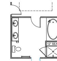
LUXURY BATH OPT 7 42" x 72" GARDEN TUB 35" x 48" FIBERGLASS SHOWER LOSE 2' FROM MASTER BR
