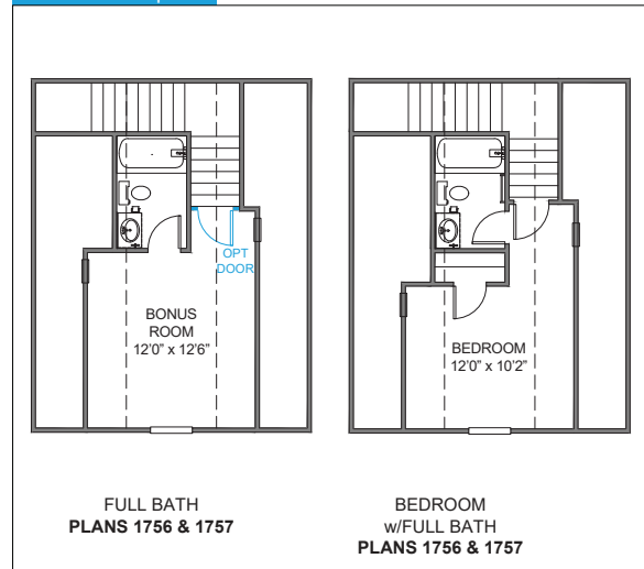
Bonus Room Options
